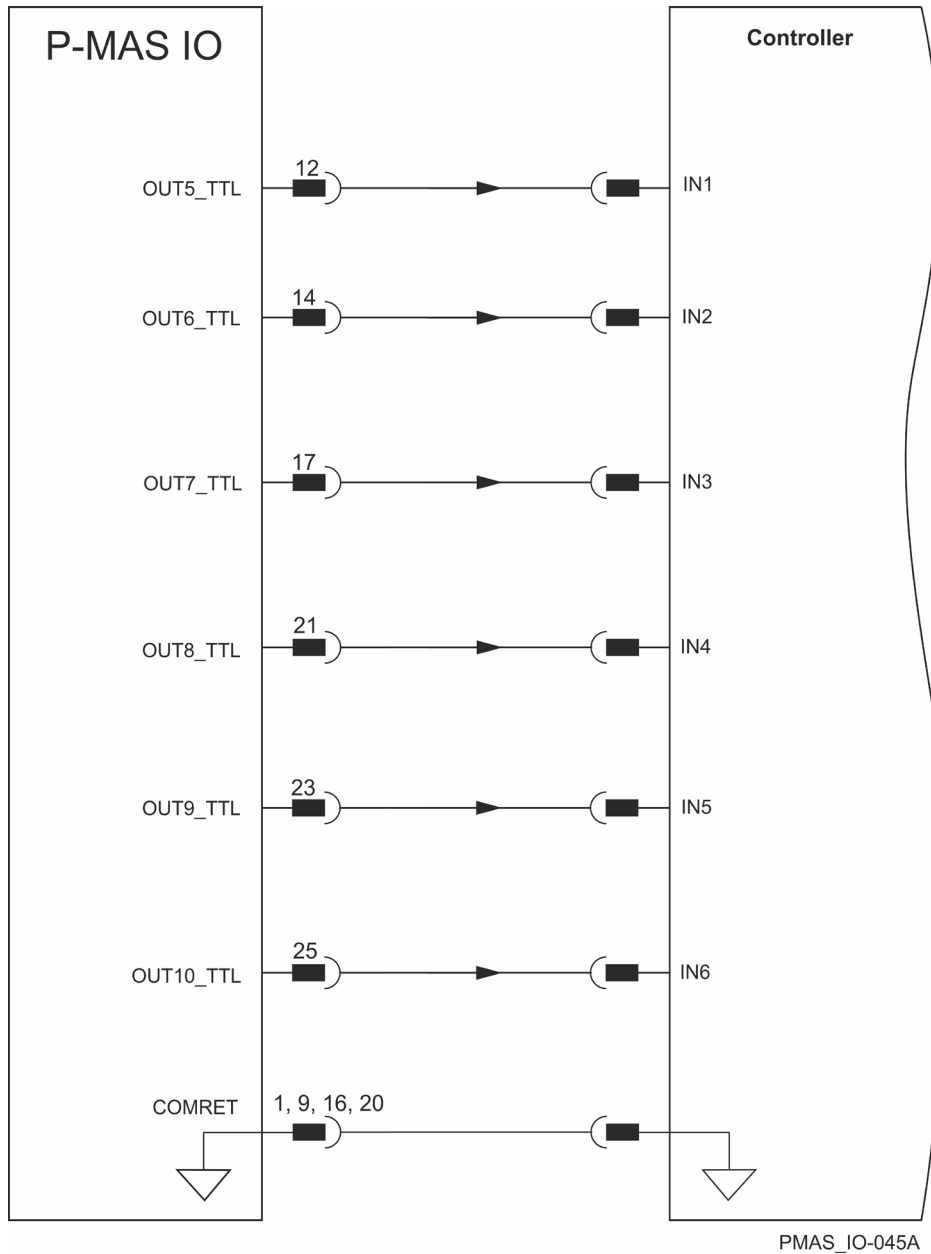
Figure 21: Single Ended Outputs Connection Diagram
