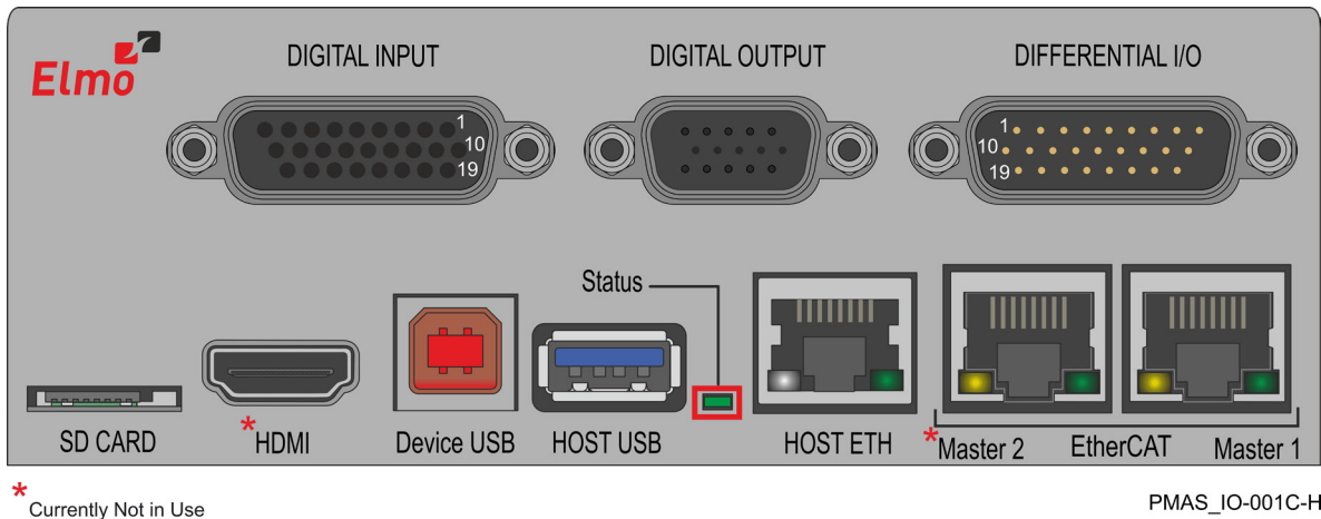
Figure 4: Platinum Maestro Status Indicator
