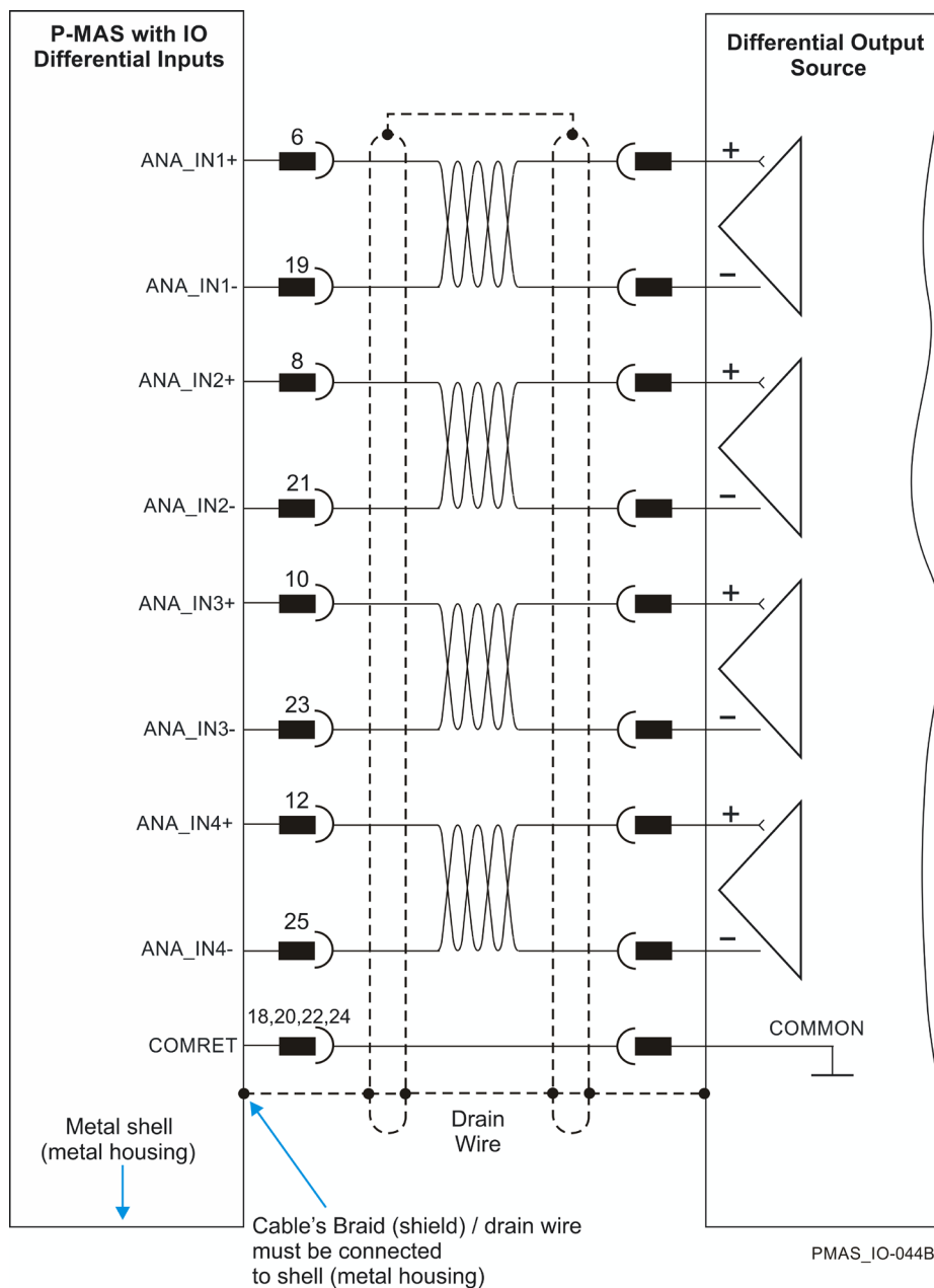
Figure 23: Differential Analog Input Connection Diagram
