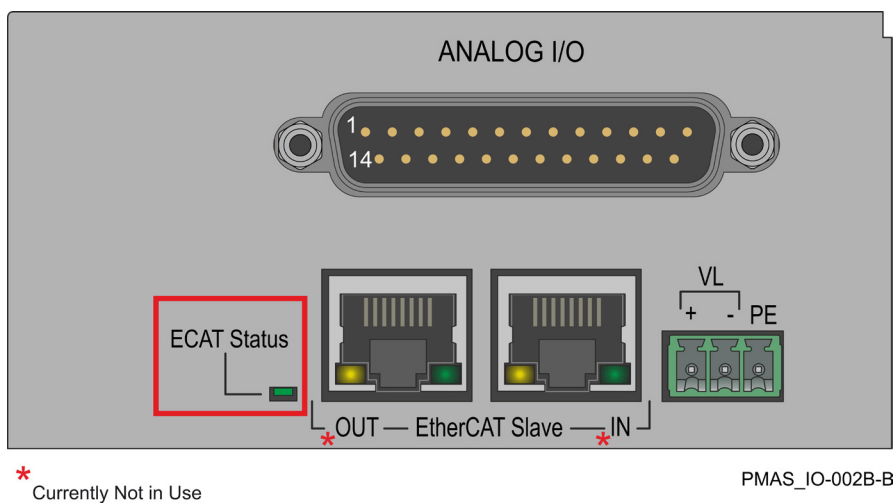
Figure 6: EtherCAT Status LEDs
