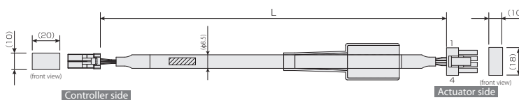
(Fig.: Motor robot cable CB-X2-MA□□□□ with plastic connector)
